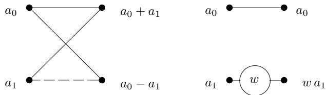
Figure 13: Signal flow graphs of \mathbf{F}_2 \mathbf{a} and \text{diag}(1, w) \mathbf{a} .
