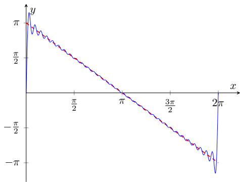
Figure 7: The convolution f * D_{32} of the 2\pi -periodic sawtooth function f and the Dirichlet kernel D_{32} approximates f quite good except at the jump discontinuities (left). The convolution f * F_{32} of f and the Fejér kernel F_{32} approximates f not as good as f * D_{32} , but it does not oscillates near the jump discontinuities (right).
