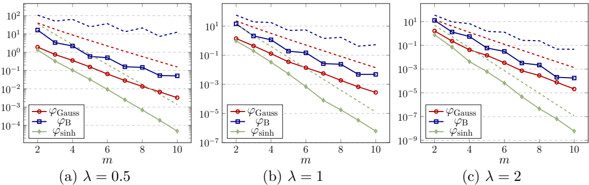
Figure 7.1: Maximum approximation error (4.6) (solid) and error constant (3.20) (dashed) using \varphi \in \{\varphi_{\text{Gauss}}, \varphi_{\text{B}}, \varphi_{\text{sinh}}\} for the function f(x) = \delta \text{sinc}^2(\delta\pi x) with N = 256 , \tau = 0.45 , \delta = \tau N , as well as m \in \{2, 3, \dots, 10\} , and \lambda \in \{0.5, 1, 2\} .
