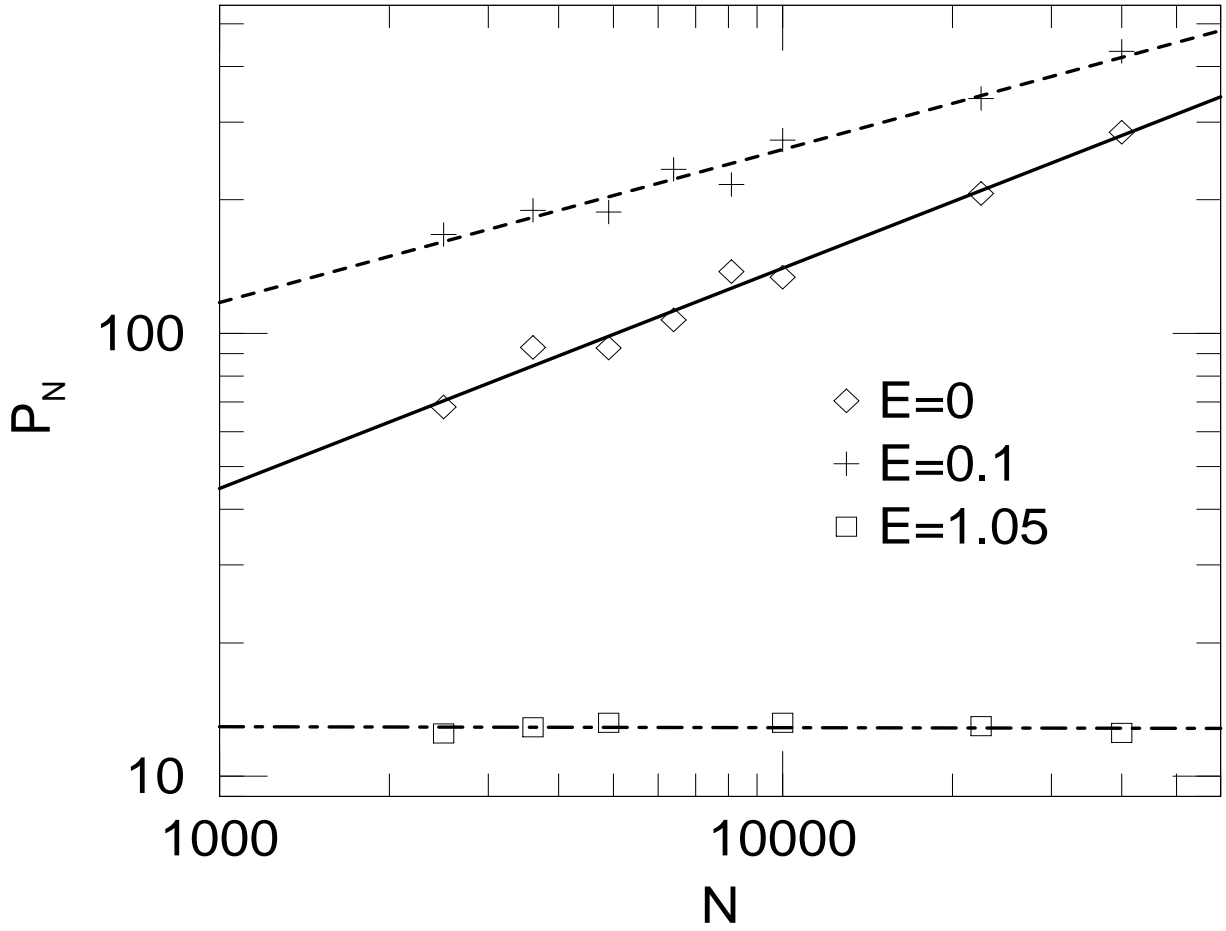
FIG. 7. Finite-size dependence of the participation numbers P_N for eigenstates with c = 0 at energies in the band center ( E = 0 ), outside the band center but still close to the peak in the DOS ( E = 0.1 ), and close to the band edge ( E = 1.05 ).
