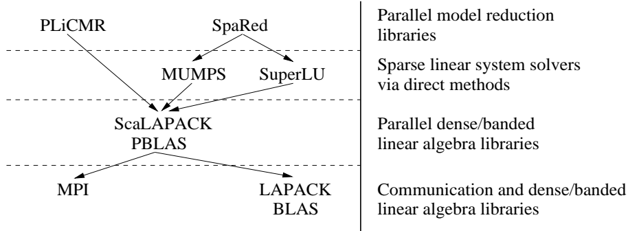
Figure 2: Multilayered architecture of libraries for model reduction.
