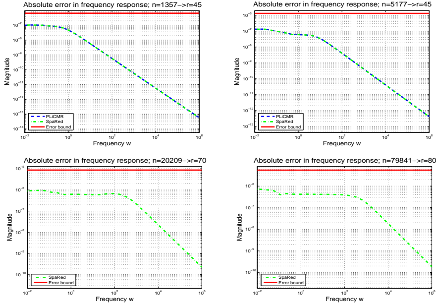
Figure 3: Absolute error in the frequency response for the reduced-order realizations.
