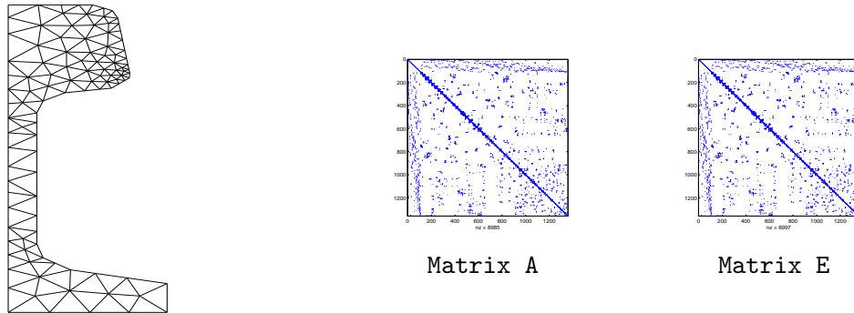
Figure 1: Finite element discretization of the profile (left) and sparsity pattern (right) for the model of order n=1,357 .
