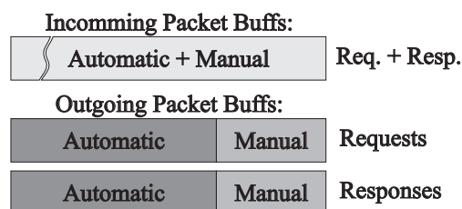
Figure 1: GPSB Packet Buffers
