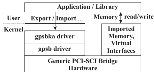
Figure 2: Layered architecture of System Software
