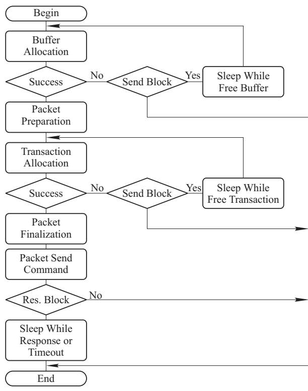
Figure 3: Generic block diagram of the request-send functions
