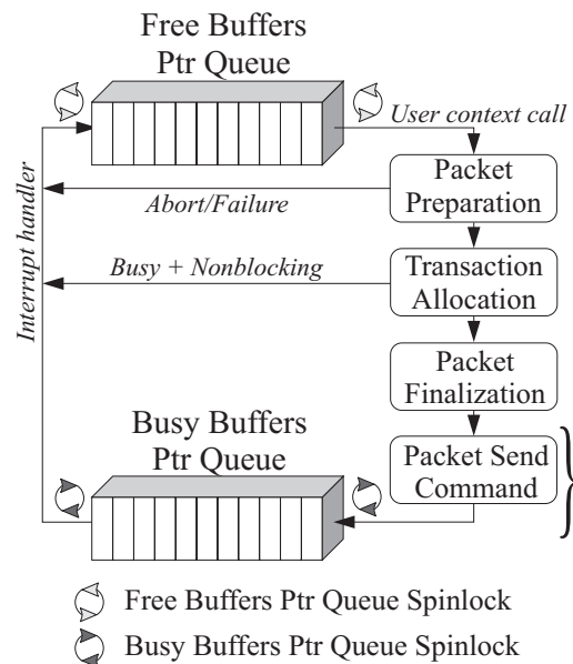
Figure 4: Request-Send Buffers Management
