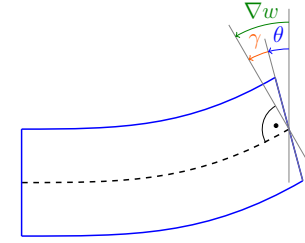
Figure 2: Deformed plate from one side; thickness exaggerated
