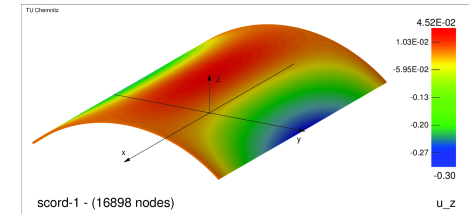
Figure 5: Scordelis–Lo roof with vertical deflection u_z^{3D}
