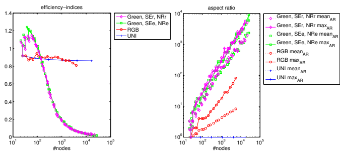
Figure 16: Comparison of different refinement algorithms for Example 3 (c): error and indicator, efficiency, aspect ratios.
