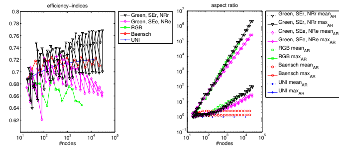
Figure 22: Comparison of different refinement algorithms for Example 5: error and indicator, efficiency, aspect ratios.
