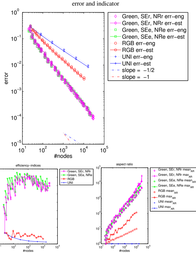
Figure 14: Comparison of different refinement algorithms for Example 3 (a): error and indicator, efficiency, aspect ratios.
