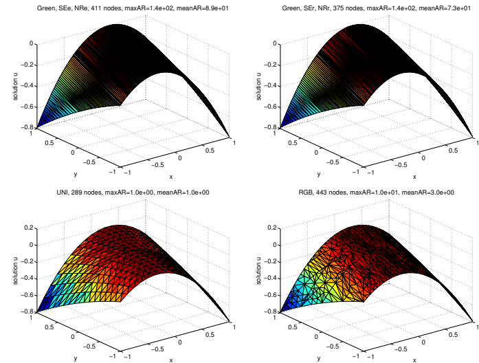
Figure 17: FE solution on meshes resulting from different refinement algorithms for Example 3 (a)
