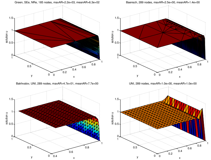
Figure 24: FE solution on meshes resulting from different refinement algorithms for Example 6 with \kappa = 10^4
