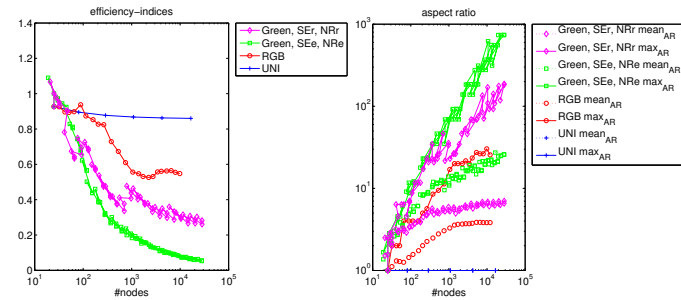
Figure 15: Comparison of different refinement algorithms for Example 3 (b): error and indicator, efficiency, aspect ratios.
