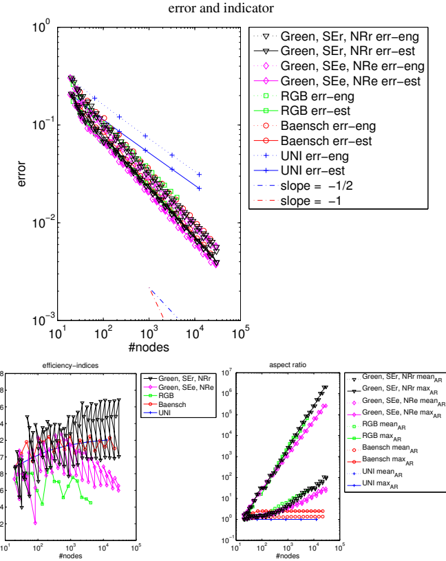
Figure 22: Comparison of different refinement algorithms for Example 5: error and indicator, efficiency, aspect ratios.
