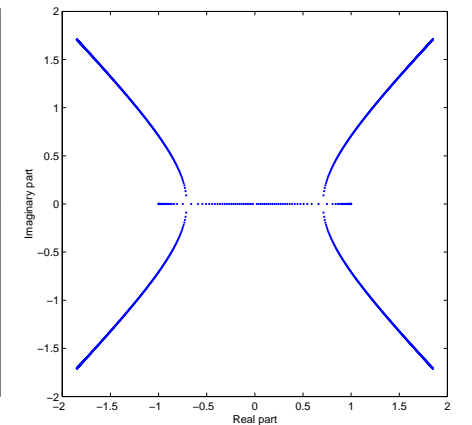
Figure 3.2: Spectrum of the test matrix
