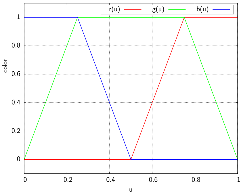
(b) Color mapping functions
