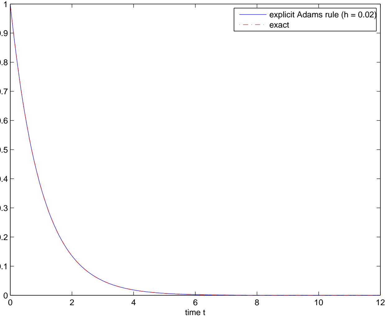
Exact solution y(t) = \exp(-t) and solution by explicit twostep Adams rule
