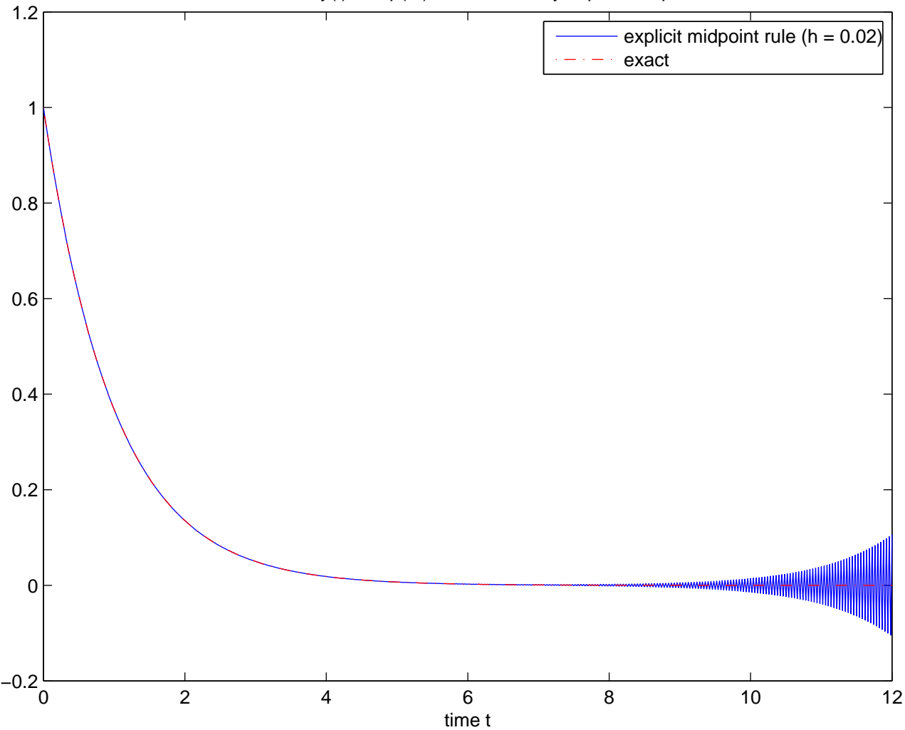
Exact solution y(t) = \exp(-t) and solution by explicit midpoint rule
