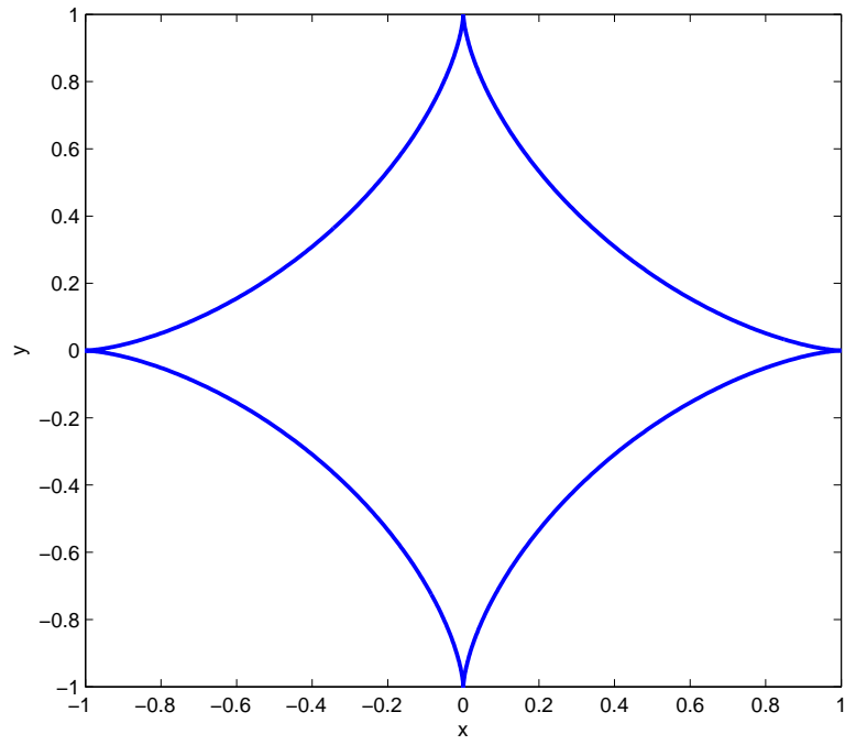
Astroide, a = 1
