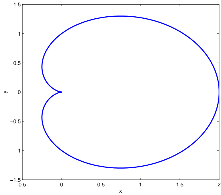
Kardioide, a = 1
